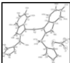
Fig. 1. View of the title complex, showing the labeling of the 30% probability ellipsoids.
